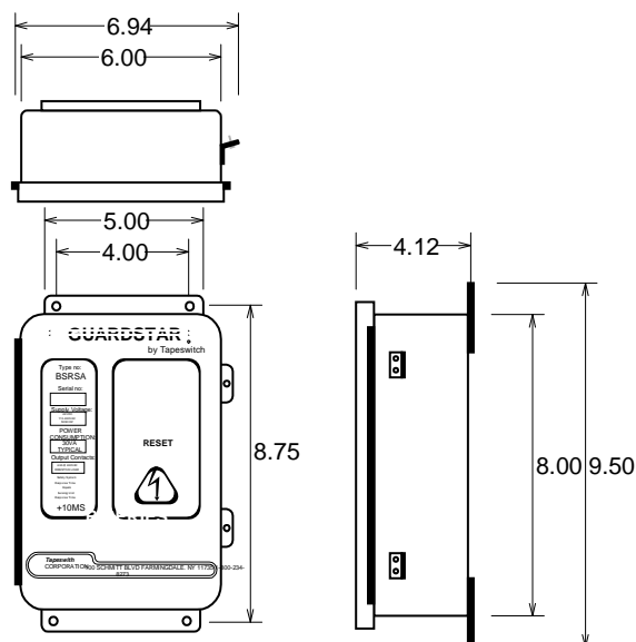
Figure 26 – BSRSA Interface Unit Outline and Dimensions
