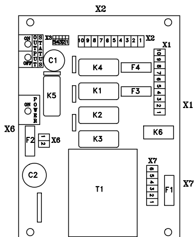
Figure 27 - BSRSA Interface Unit Internal View
