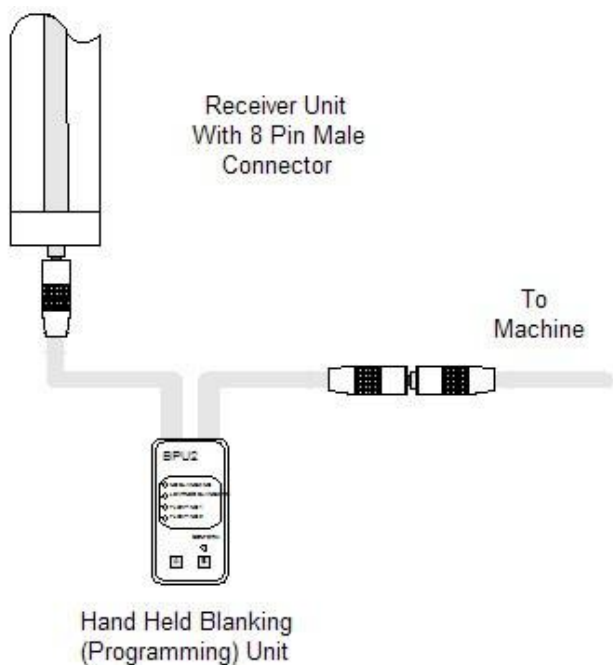
Figure 53 – BPU-2 Connected to B-Series Receiver
