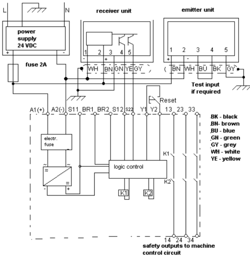
Figure 48 – SRUS Connection Details
