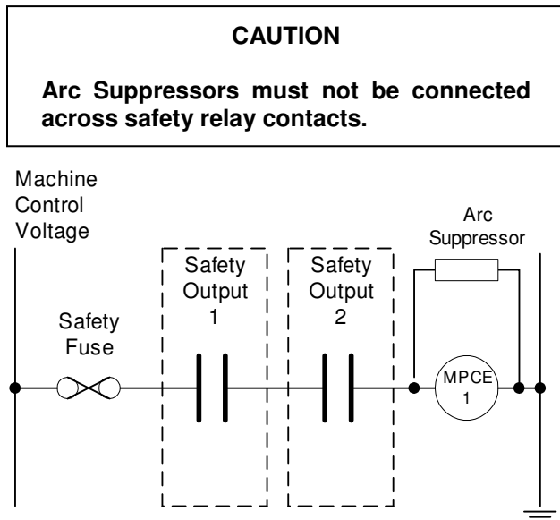
Figure 23 – Interfacing a Machine with 1 MPCE
