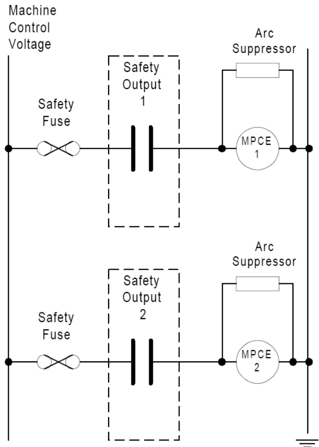
Figure 2 - Interfacing a Machine with Dual Identical MPCE's
