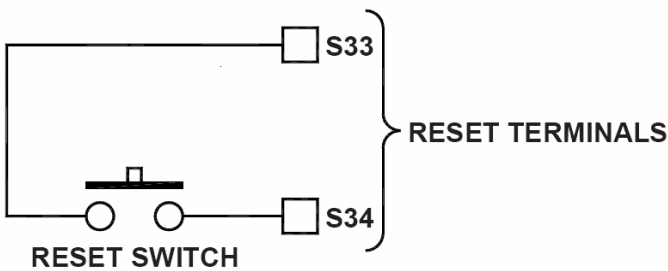
Figure 5 – Manual Reset
